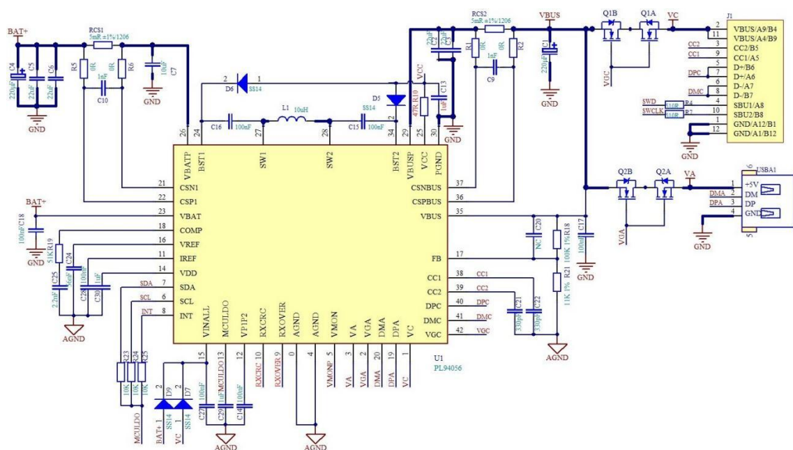
Fig. 11-2-1 Schematic
