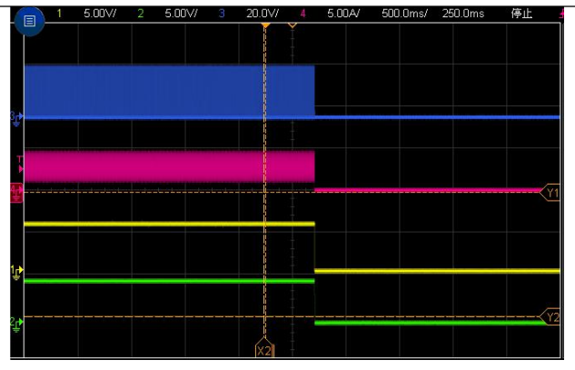
CH1: EN CH2:VOUT CH3:SW CH4:IL Vin=24V Vout=5V Shut Down waveform through EN, Iout =3A
