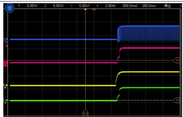
CH1: VIN CH2:VOUT CH3:SW CH4:IL Vin=5V Vout=5V Start up waveform through Vin, Iout =3A
