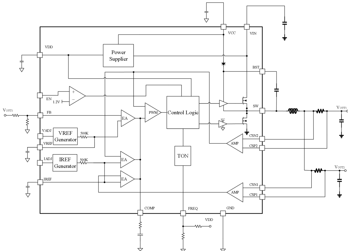
Fig. 9.1-1 Block Diagram
