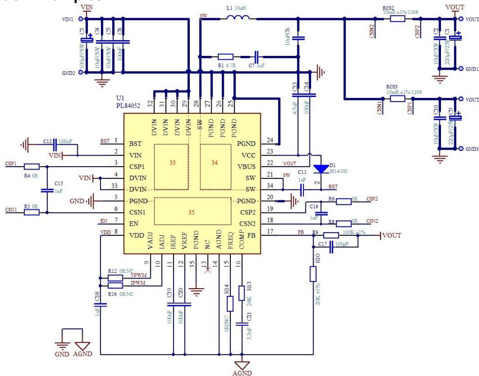
Fig. 11.2-1 Application Schematic
