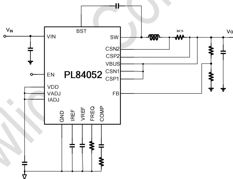
Fig. 4-1 Application Schematic
