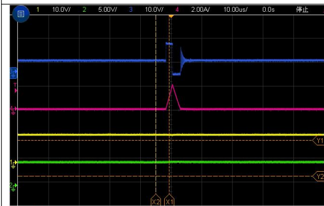
CH1: VIN CH2:VOUT CH3:SW CH4:IL Vin=5V Vout=5V Steady State waveform Iout =0A
