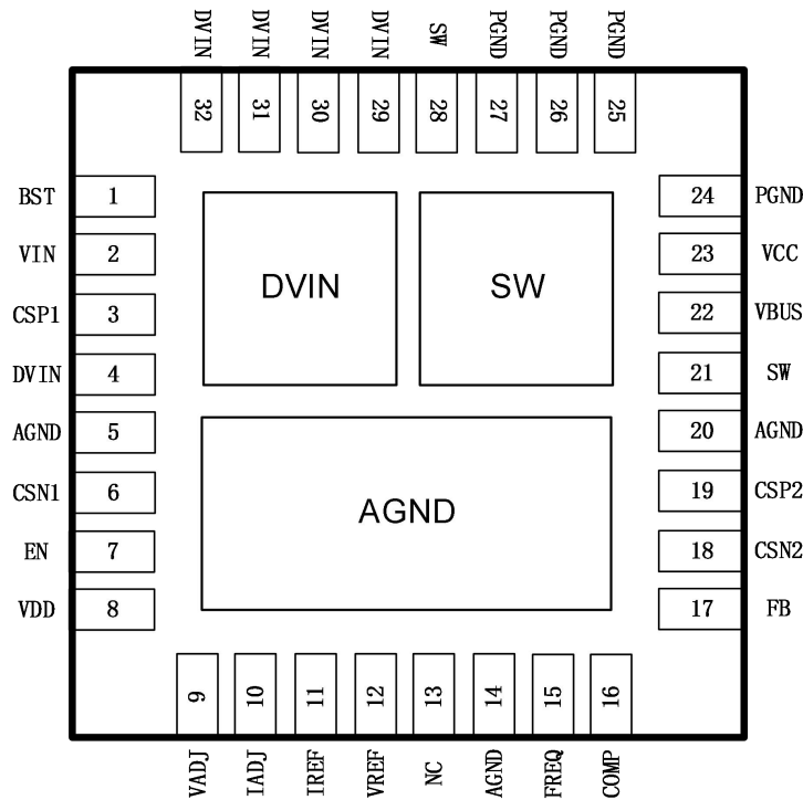
Fig. 5-1 Pin-Function (QFN5x5-32)
