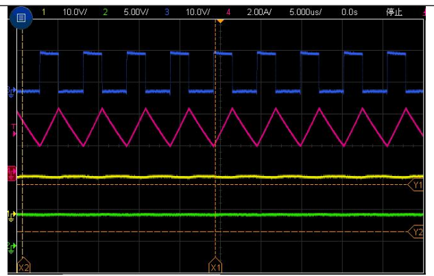
CH1: VIN CH2:VOUT CH3:SW CH4:IL Vin=12V Vout=5V Steady State waveform Iout =3A
