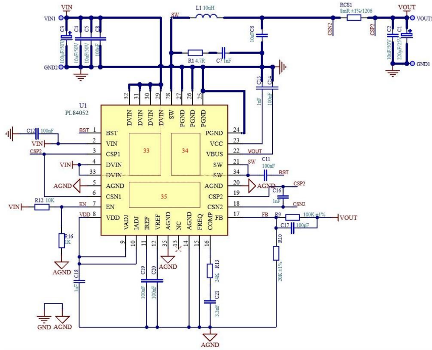
Fig. 11.2-4 Application Schematic
