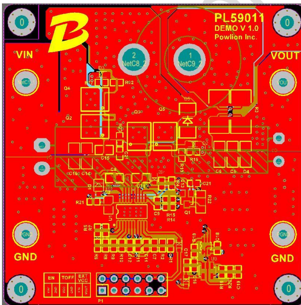
Figure 24. Top lay
