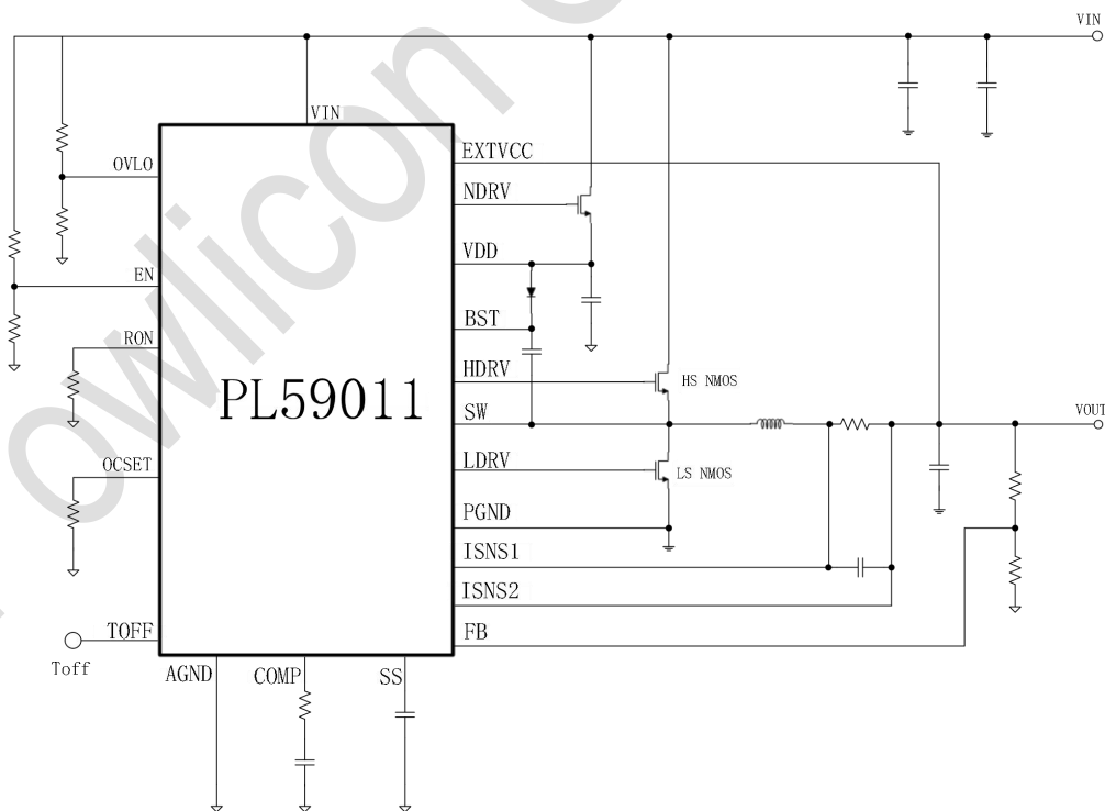
Fig. 1 Simplified Schematic
