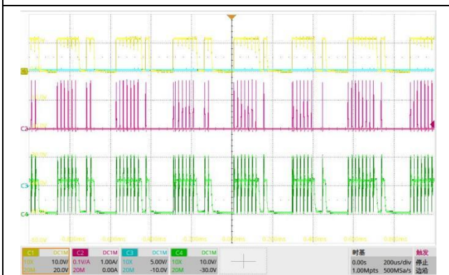
Fig.8-15 Start up waveform, Iout =1A
