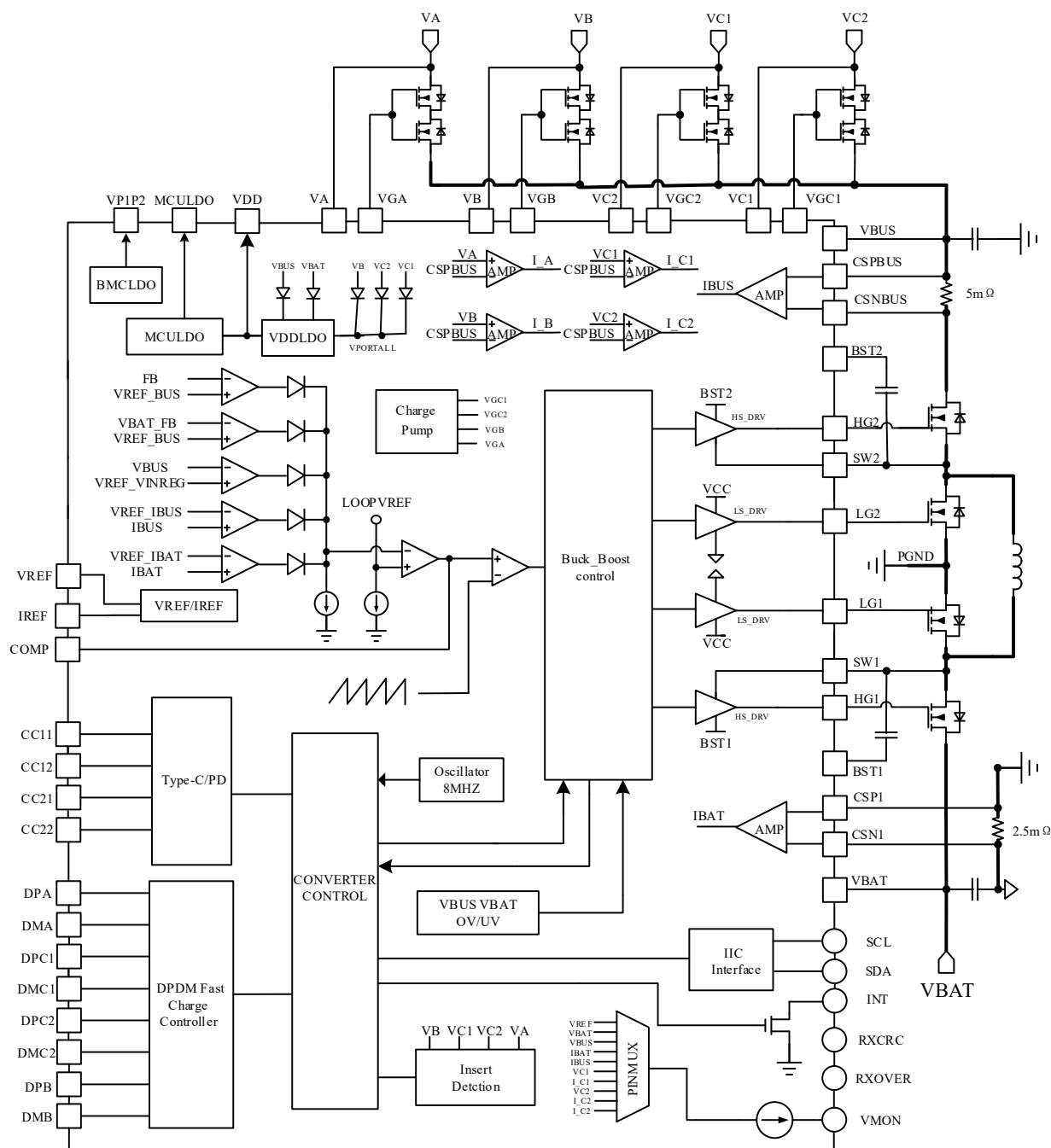
Fig. 9-2-1 PL62100 Block Diagram
