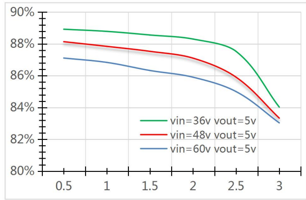
Fig.8-2 Efficiency
