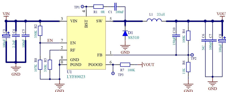
Fig. 11-2-1 Schematic
