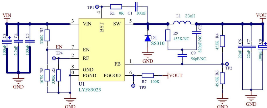
Fig. 11-2-2 Schematic
