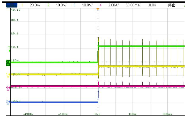
Fig.8-7 Start up waveform through EN, Iout =0A
