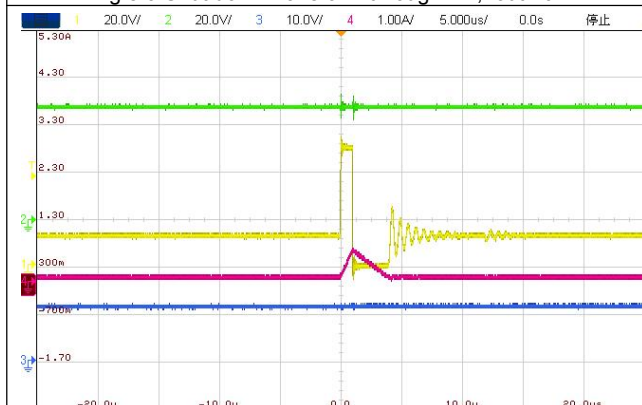
Fig.8-9 Shut down waveform through EN, Iout =0A
