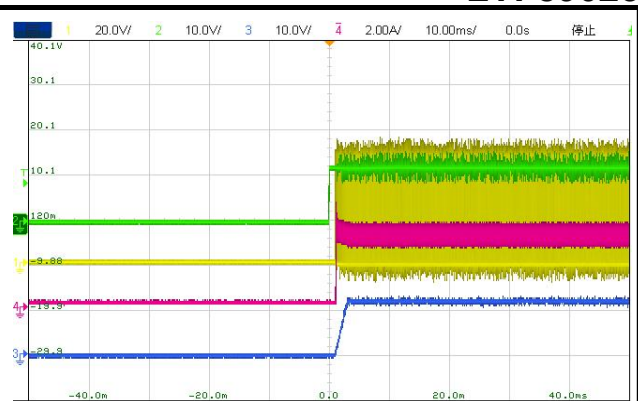
Fig.8-8 Start up waveform through EN, Iout =3A
