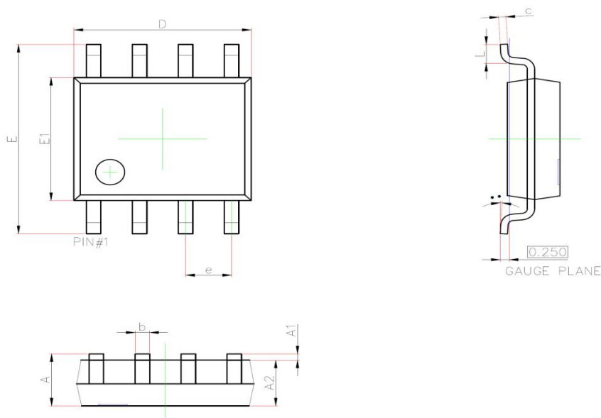
SOP8PACKAGE OUTLINE DIMENSIONS
