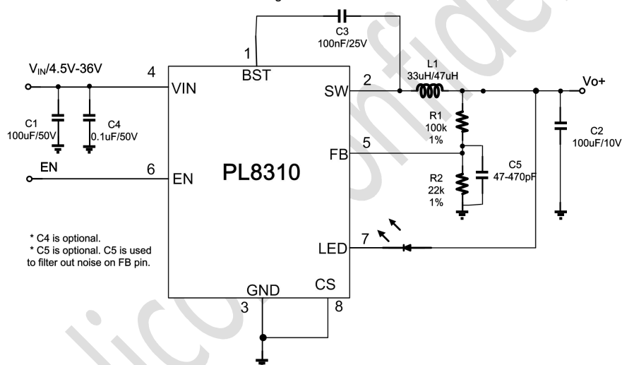
Work Mode2: CS to GND
