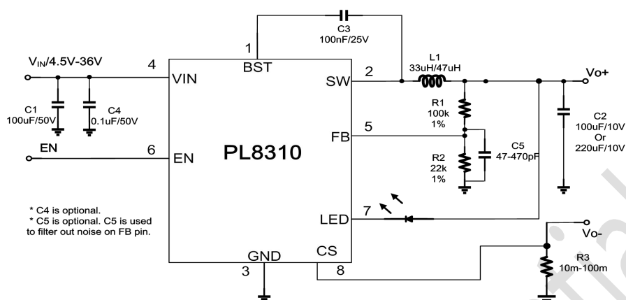
Work Mode 1: CS to GND with sensing resistor Fig. 1 Schematic
