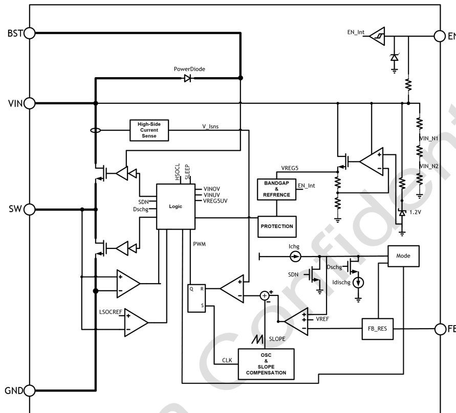
Fig.22 PL88102 Diagram
