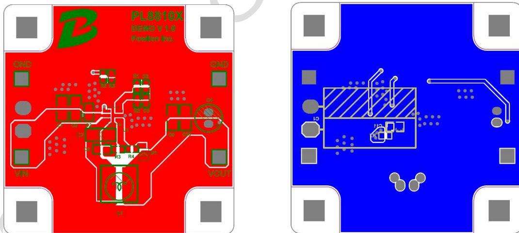
Fig 25 PCB Layout
